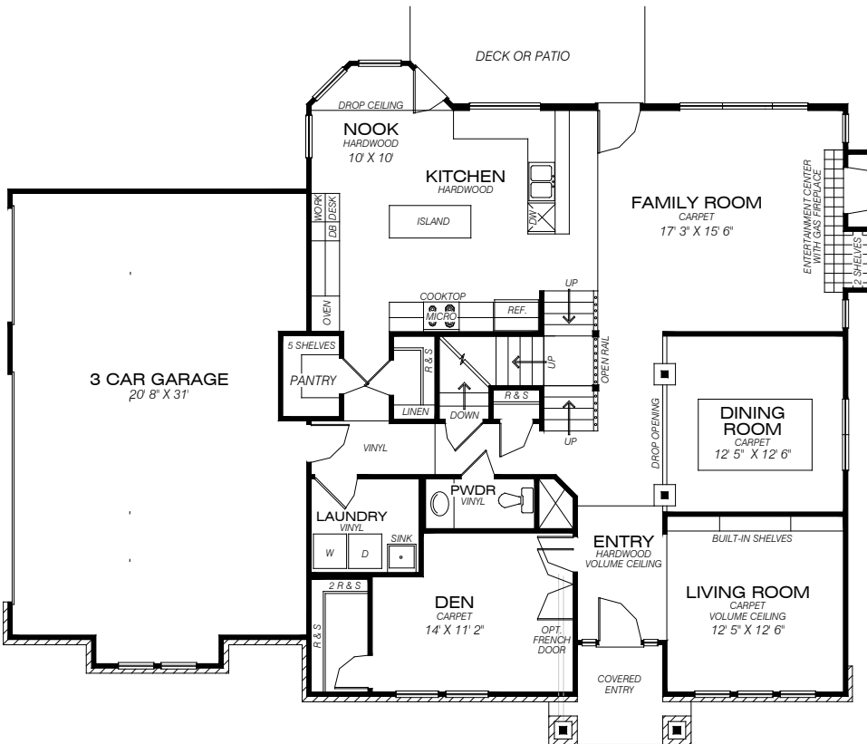
SIDE LOAD GARAGE
