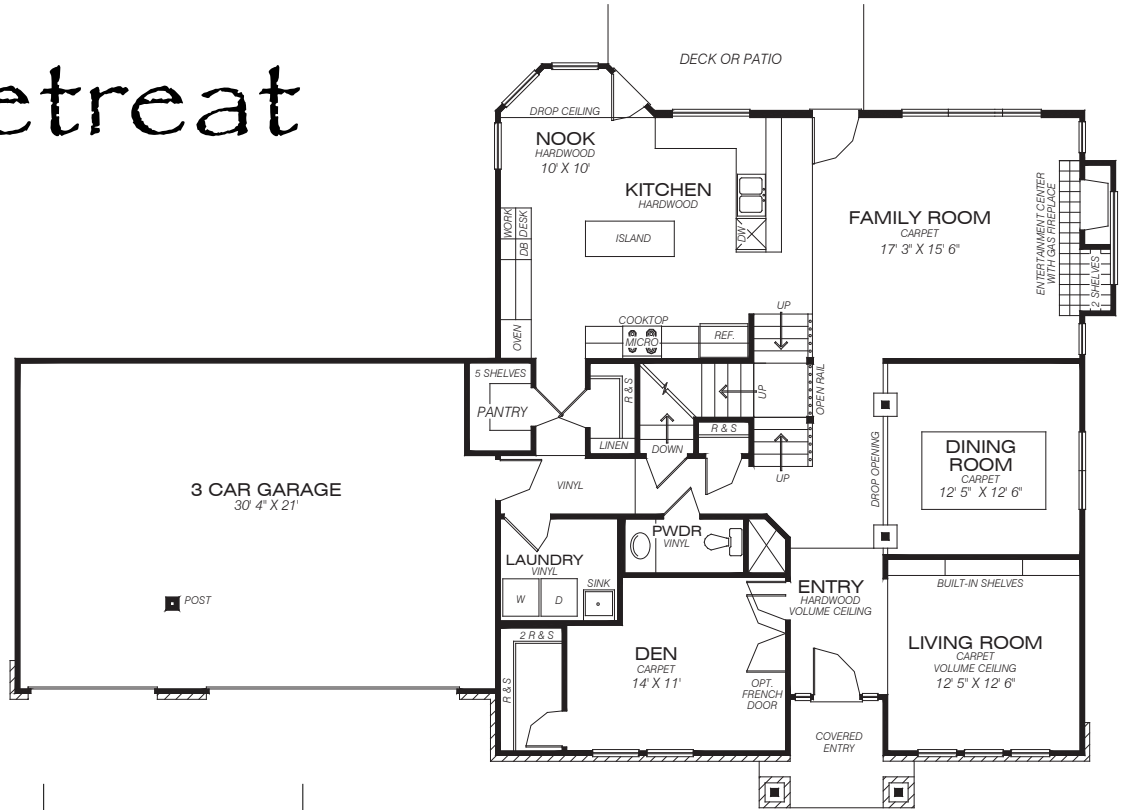
FRONT LOAD GARAGE
