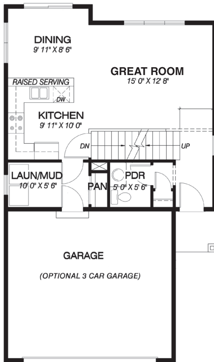
MAIN LEVEL
